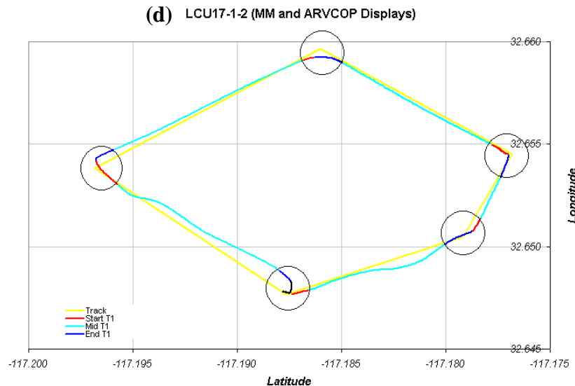
Figure 7. Plots of sample LCU runs, each using one of the test configurations: a) paper chart for navigator; b) moving-map for navigator; b) moving-map for navigator and craftmaster; c) moving-map for both and ARVCOP for craftmaster.
