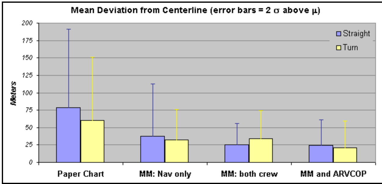
Figure 8. Cross-track error of sample LCU runs.
