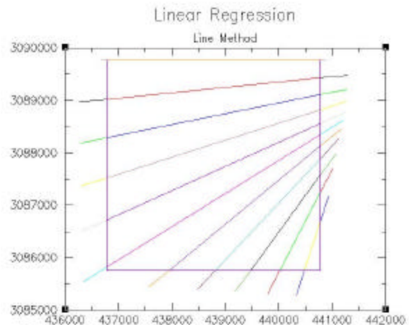
Fig. 2 Lines generated using the LR line method. The coordinate system is in meters. Notice that this method retains the use of straight lines but is no longer constrained to lines that are parallel.
