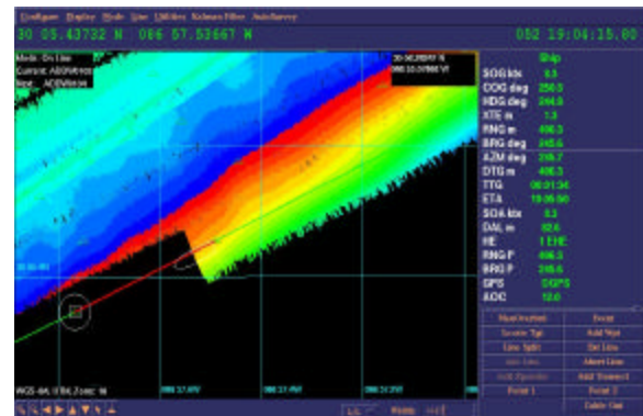
Fig. 5 A screen capture of an AutoSurvey mission running on ISS-60. The survey area was 20 miles south of Pensacola, FL.
