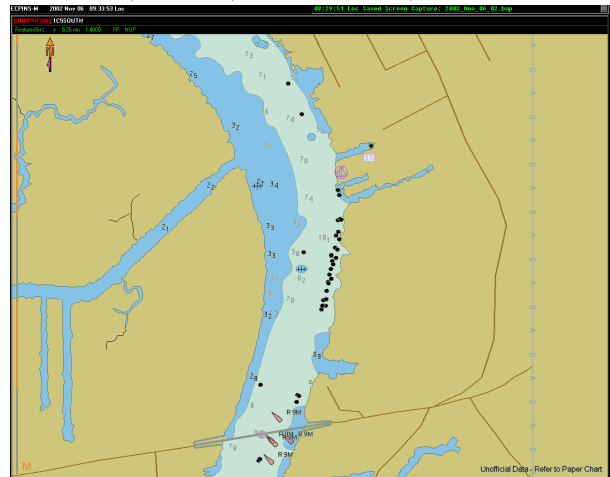
Figure 4. USM’s survey data of the Pearl River, MS
