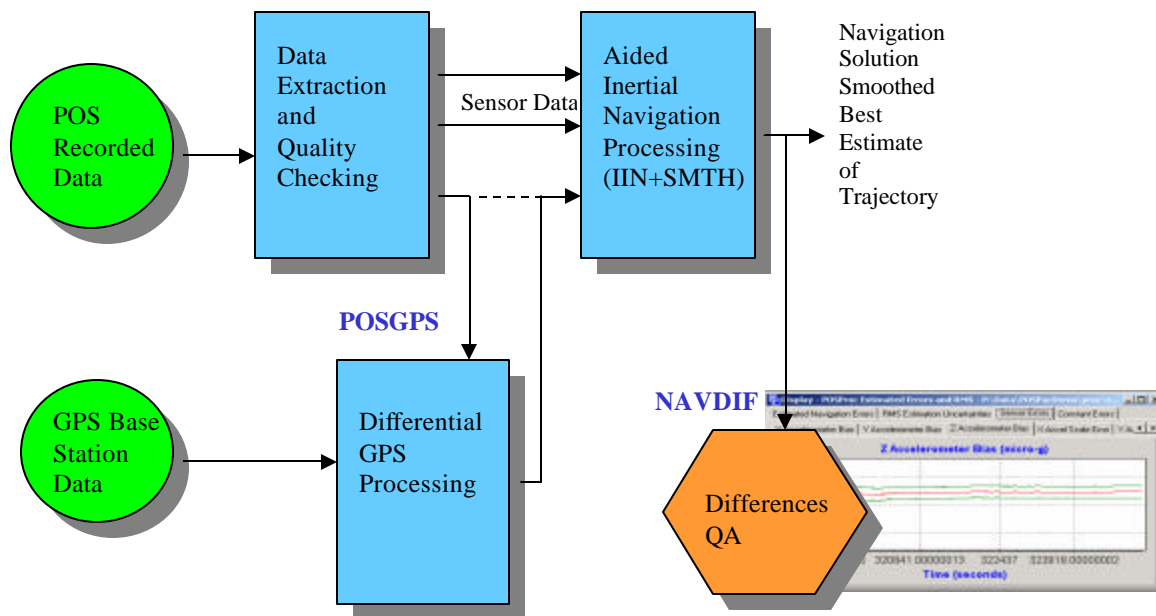
Figure 9 POS Post Processing Architecture
