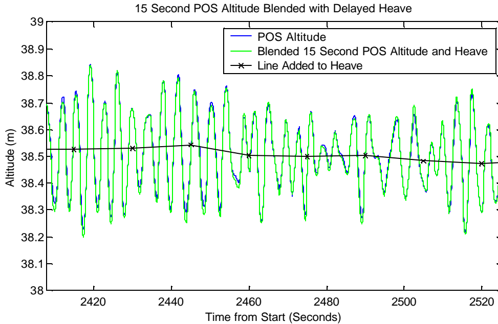
Figure 8 Outage Immunity for Vertical Positioning
