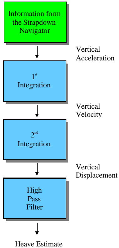
Figure 3 Double Integrated Vertical Acceleration = Heave
