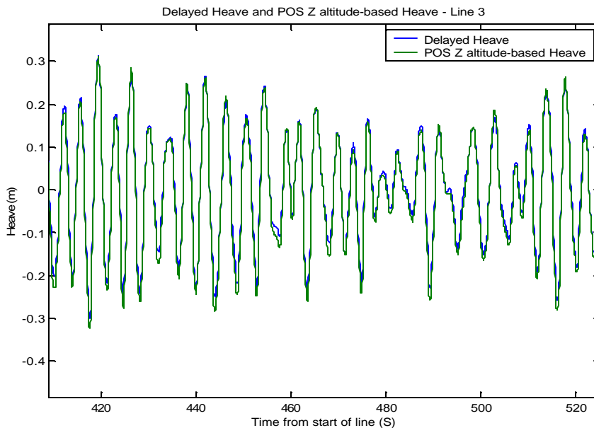
Figure 7 Inertially-Aided Kinematic GPS Z vs. the Heave Channel
