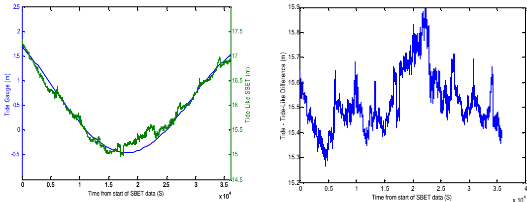
A) Plot of Tide-like channel from IARTK altitude data compared with Tide Gauge, limiting the x-axis to the IARTK data range. (Note the different y-axis ranges)
