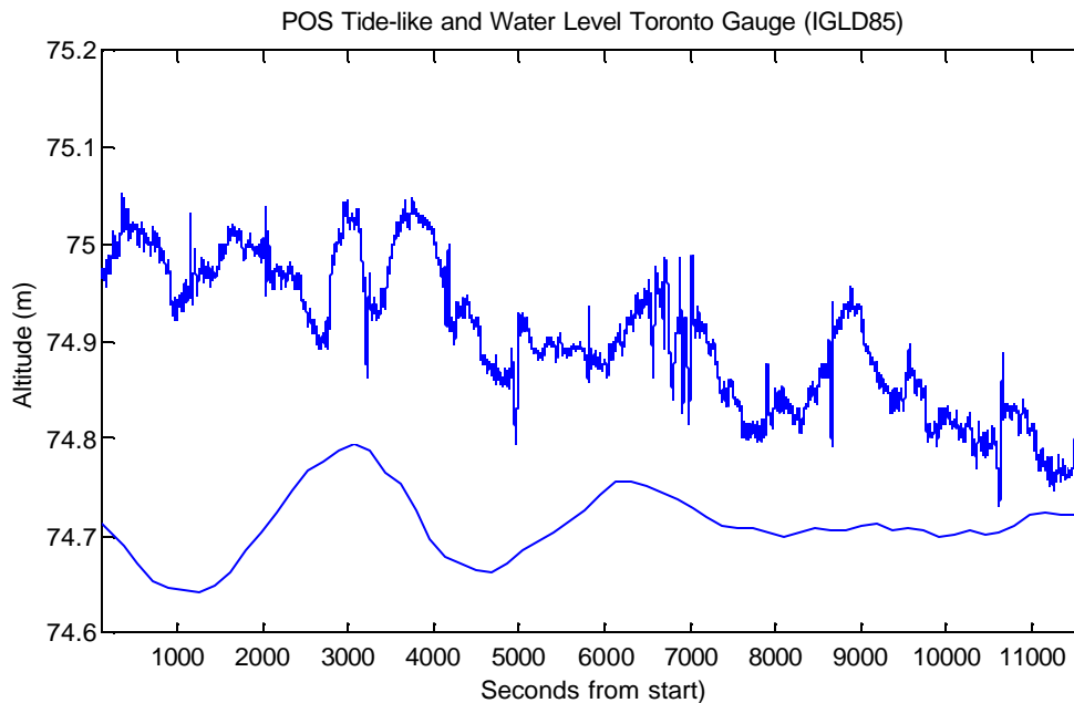
Figure 5 Seiche Effect in Lake Ontario - Measured By POS
