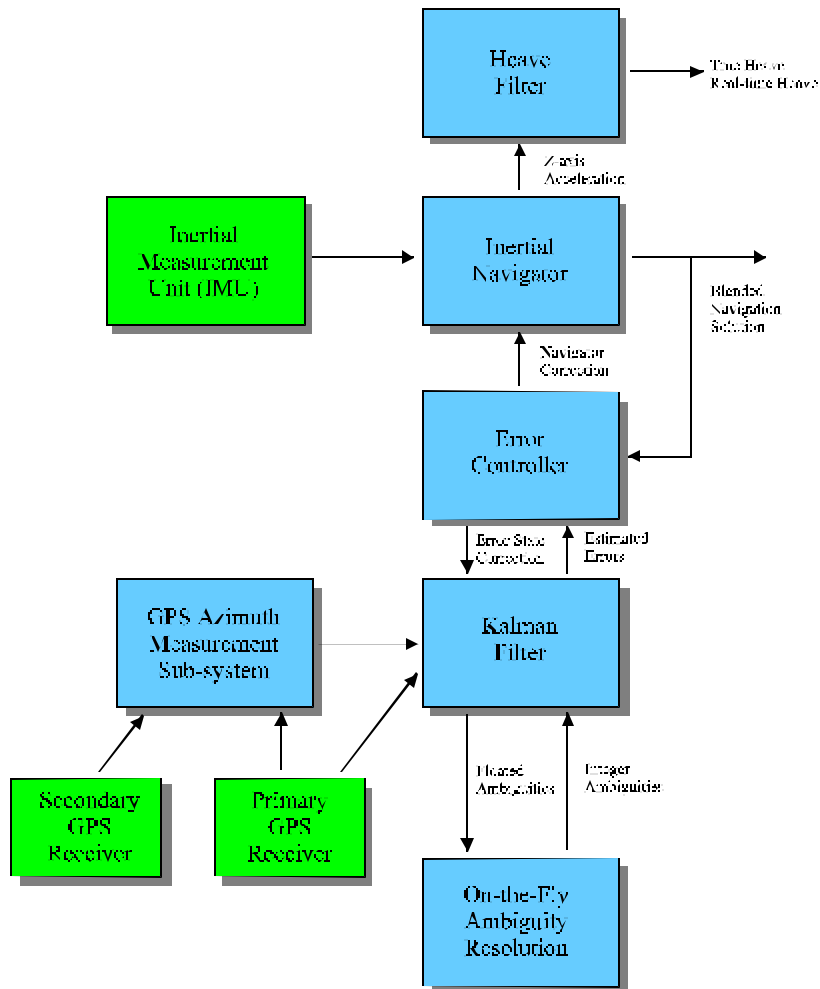
Figure 2 POS MV – Tightly-coupled Inertially-Aided RTK
